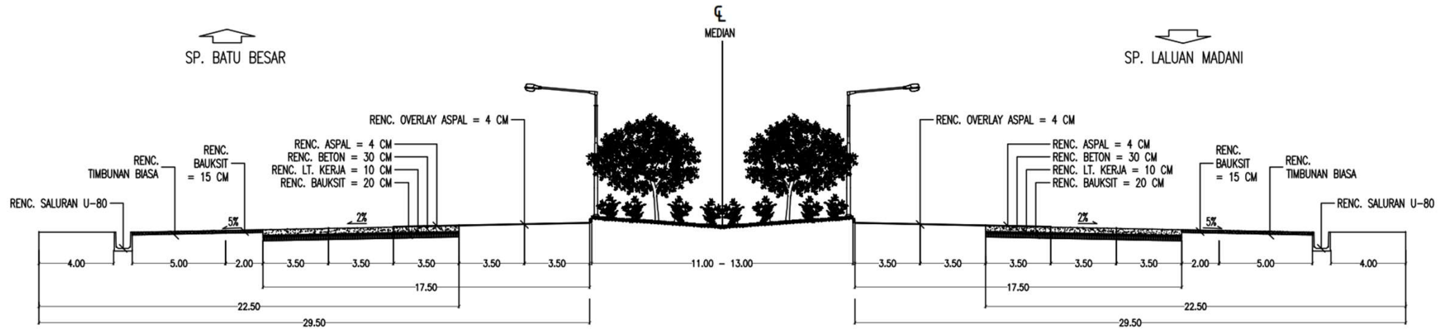
DETAIL TYPICAL JALAN HANG TUAH SKALA 1 : 100
